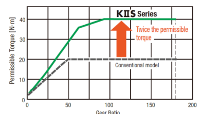
● Gearhead output (permissible) torque for 100 W
